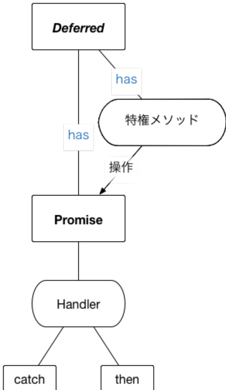
Figure 13. DeferredとPromise
